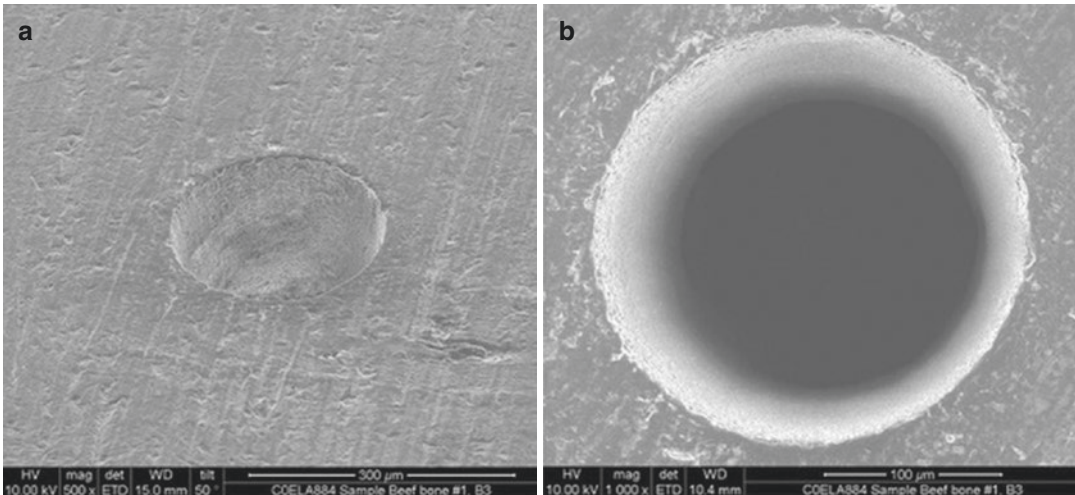
Fig. 9.3 The SEM image of a microhole generated with a femtosecond laser: (a) Overview and (b) top view, taken from [74] with permission
